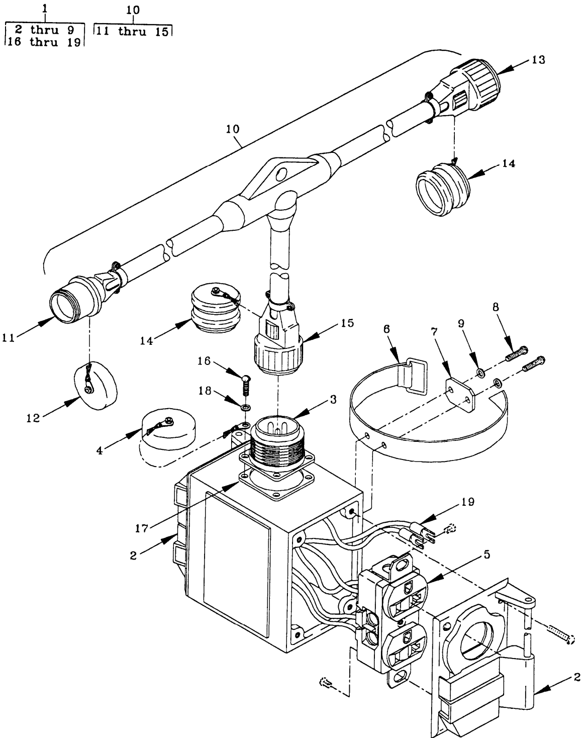
Figure 24. TYPE III/IV CONVENIENCE OUTLET
