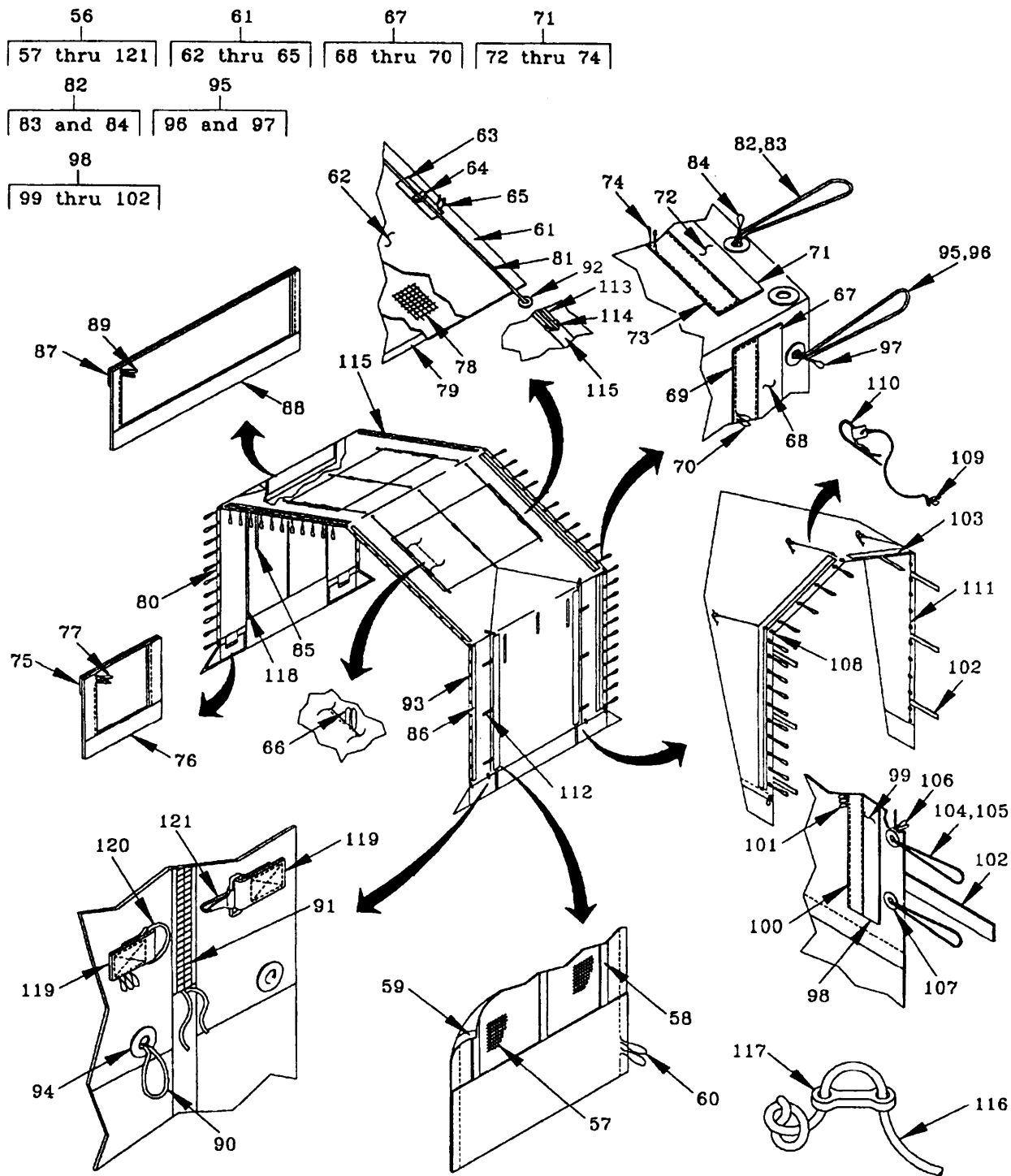
Figure 2. DOOR SECTION (Sheet 2 of 2)
