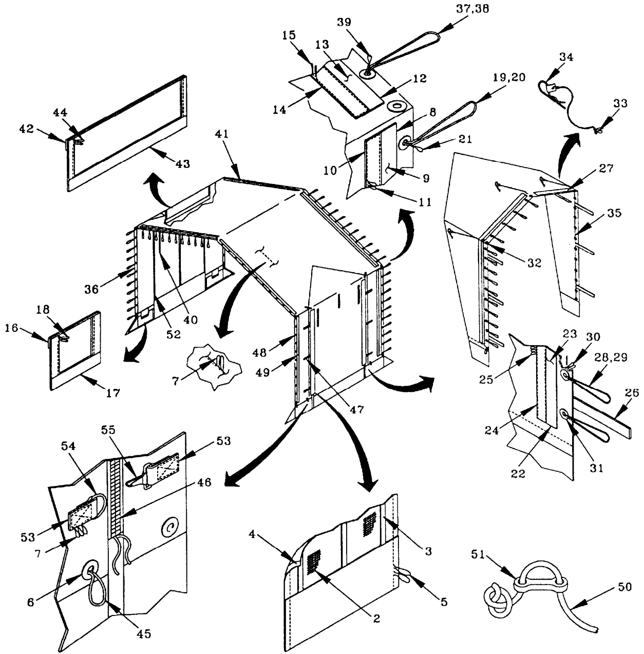
Figure 2. DOOR SECTION (Sheet 1 of 2)
