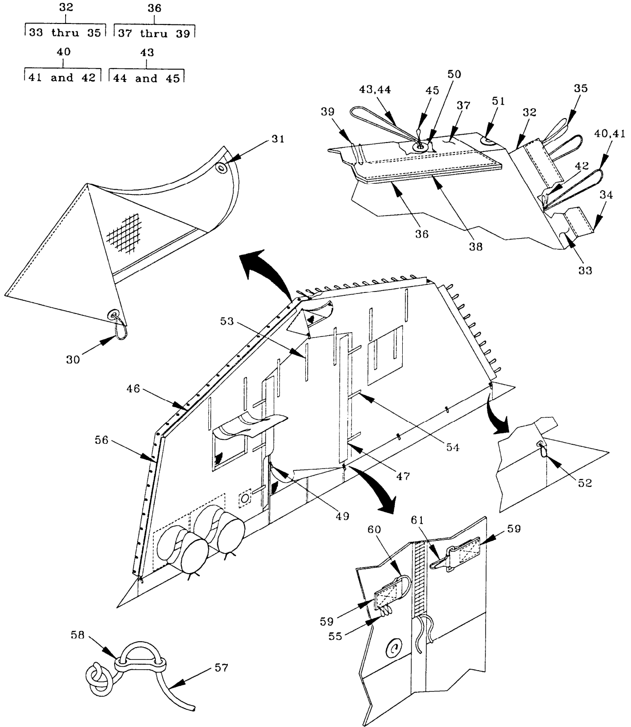
Figure 1. END SECTION (Sheet 2 of 2)
