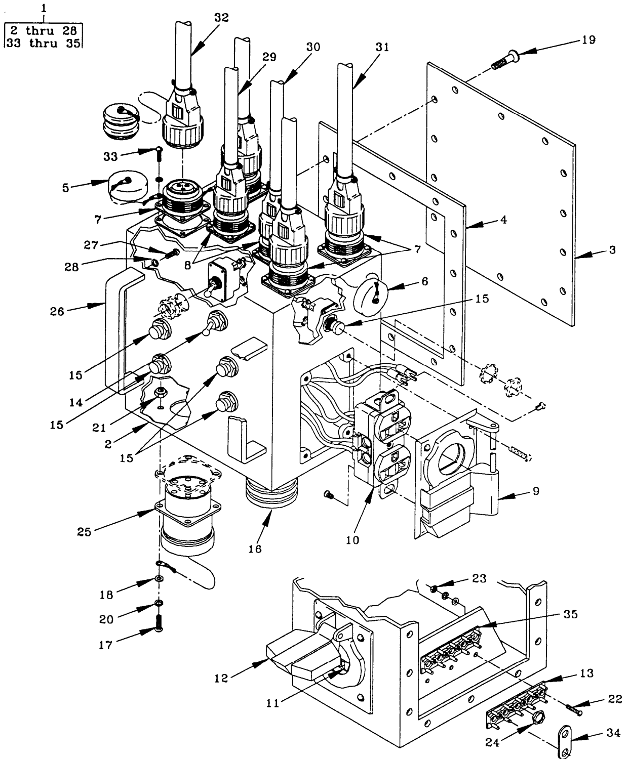
Figure 22. TYPE III POWER CONTROL
