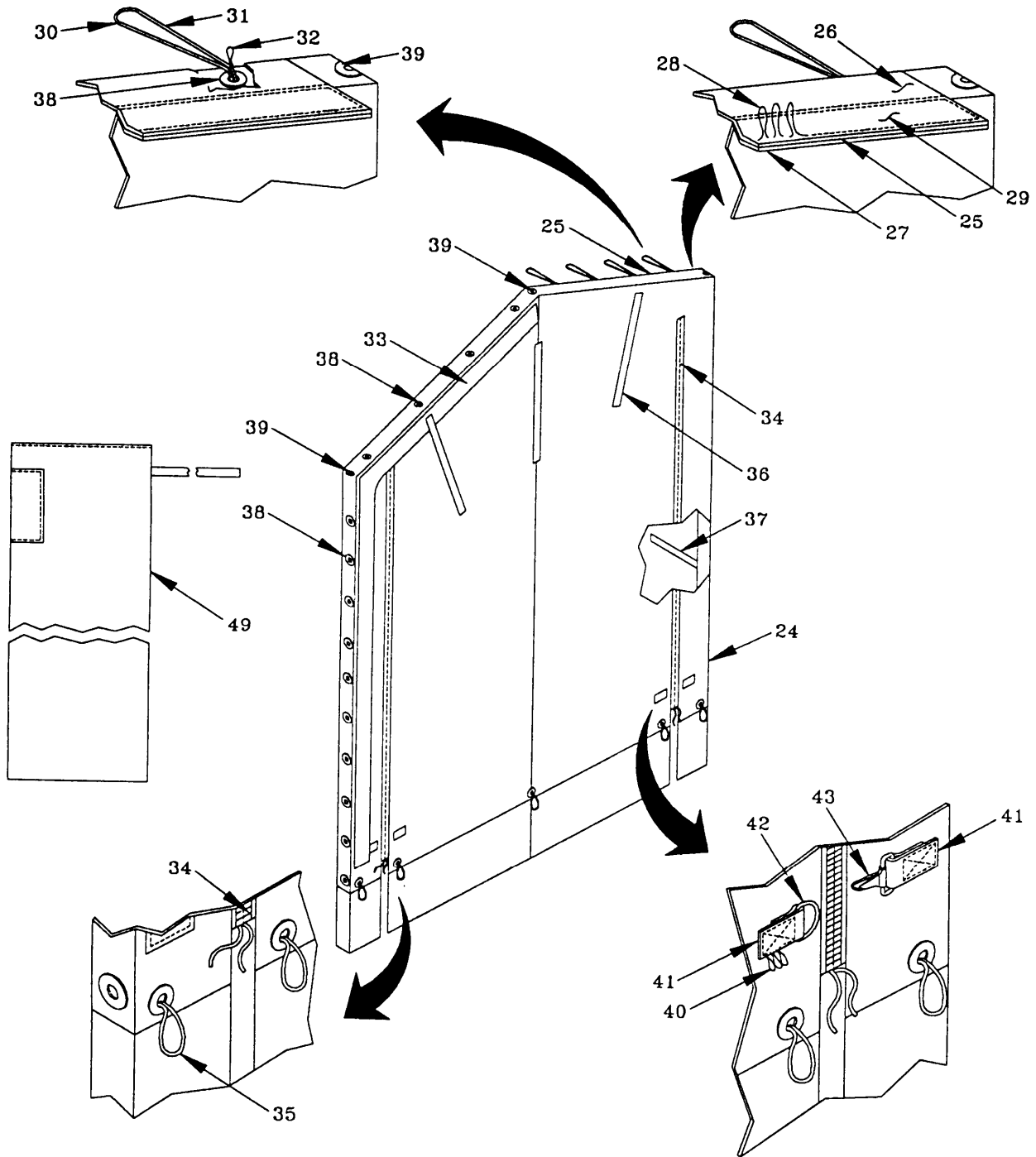
Figure 8. VESTIBULE (Sheet 2 of 2)
